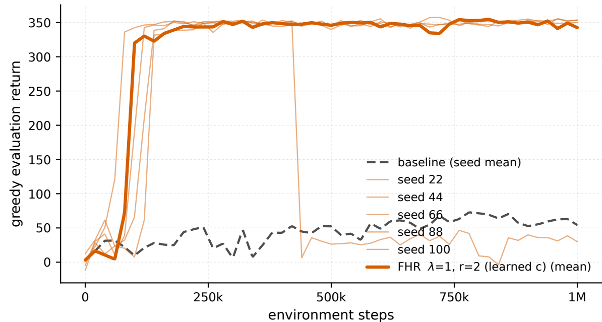
Swimmer-v5 - \lambda 1 \cdot r_2 , every seed (eval)
