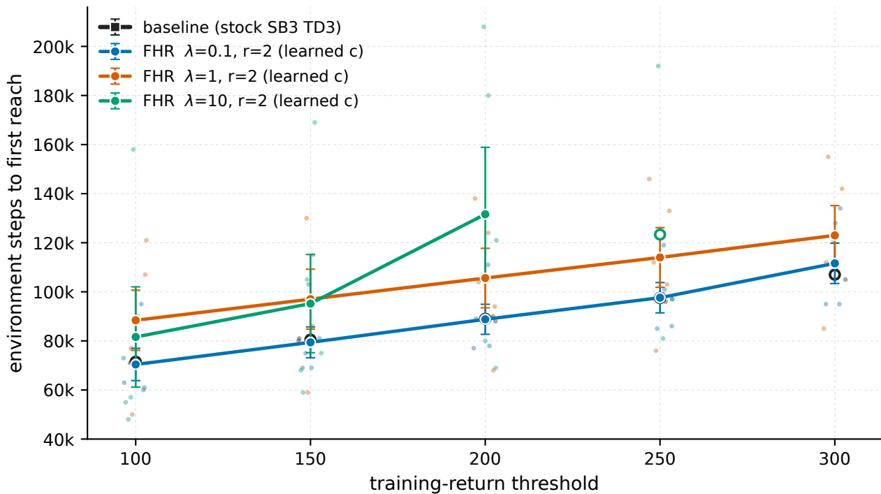
Swimmer-v5 - sample efficiency, training stream (mean \pm 1 s.e.m.) open marker: not all seeds reached it
