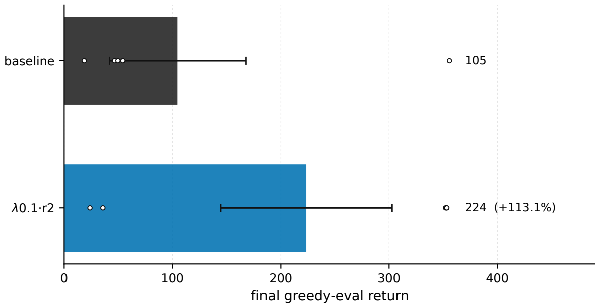
Swimmer-v5 - final return, \lambda = 0.1 vs baseline
