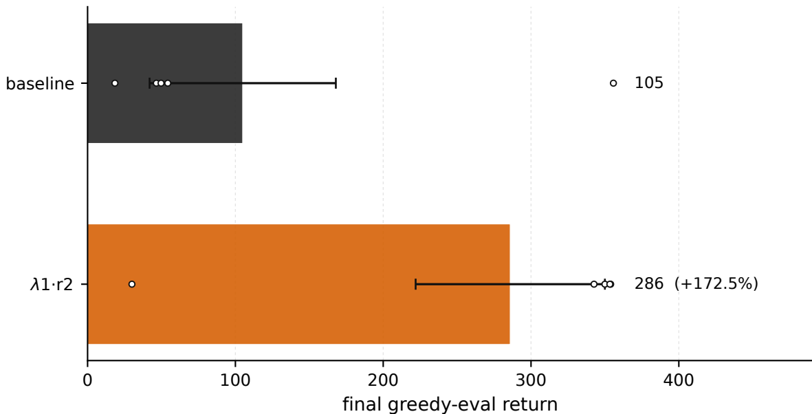
Swimmer-v5 - final return, \lambda = 1 vs baseline
