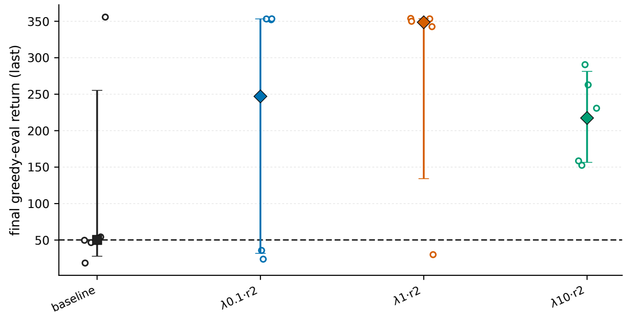
Swimmer-v5 - final return per arm: seeds (o), IQM with 95% bootstrap CI; dashed = baseline IQM
