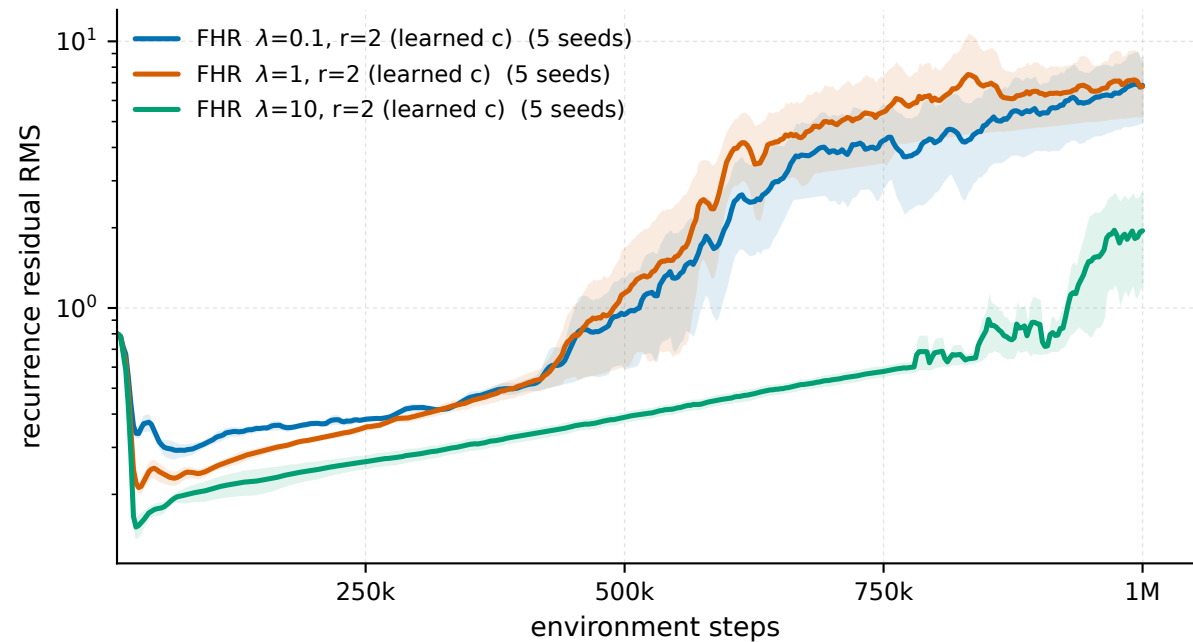
Swimmer-v5 - recurrence residual RMS
