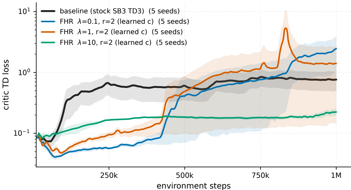
Swimmer-v5 - critic TD loss
