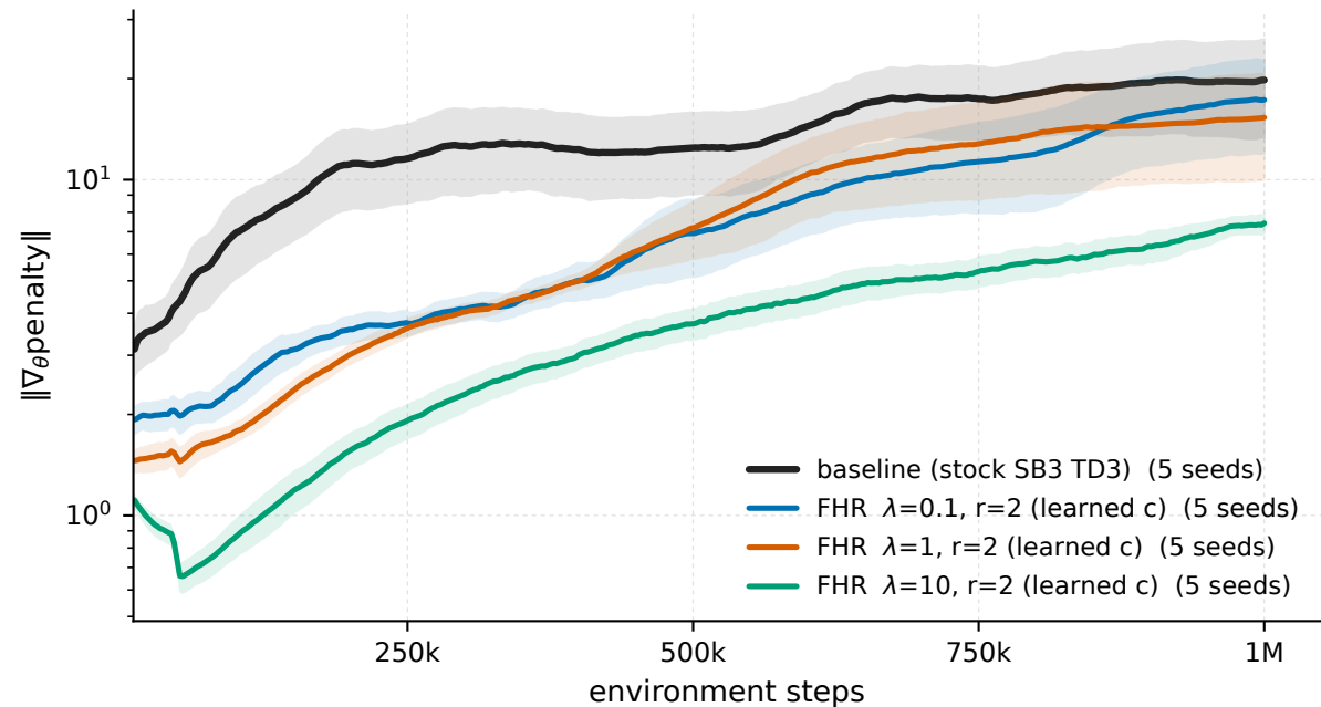
Swimmer-v5 - \|\nabla_{\theta}\text{penalty}\|
