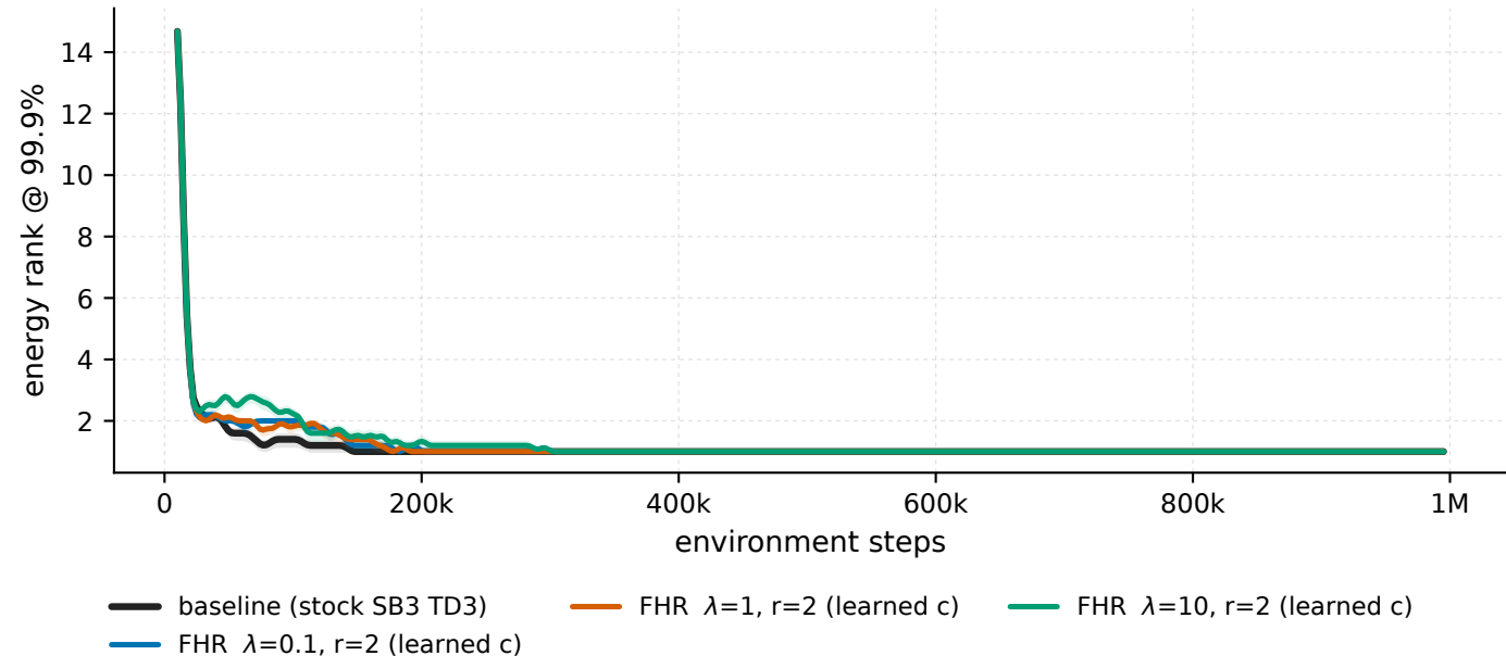
Swimmer-v5 - penalised windows, all arms energy rank @ 99.9%
