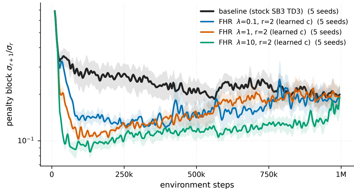
Swimmer-v5 - penalised windows: \sigma_{r+1}/\sigma_r of the penalty block
