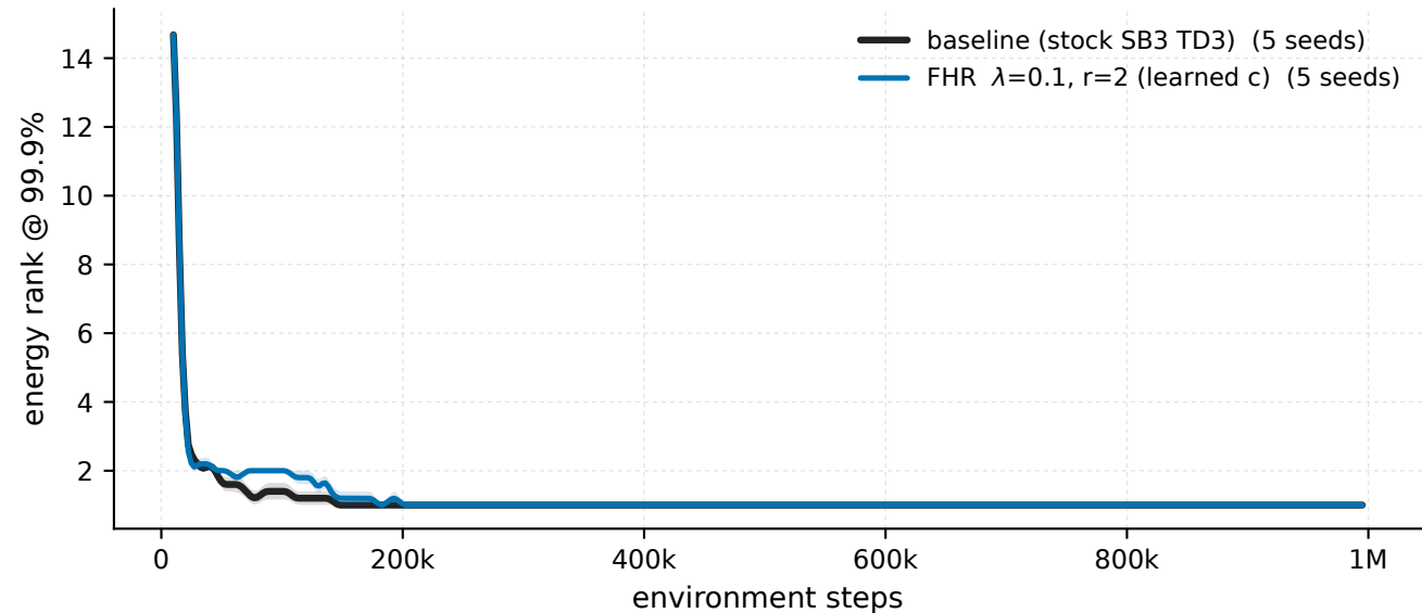
Swimmer-v5 - \lambda 0.1 \cdot r_2 vs baseline, penalised windows energy rank @ 99.9%
