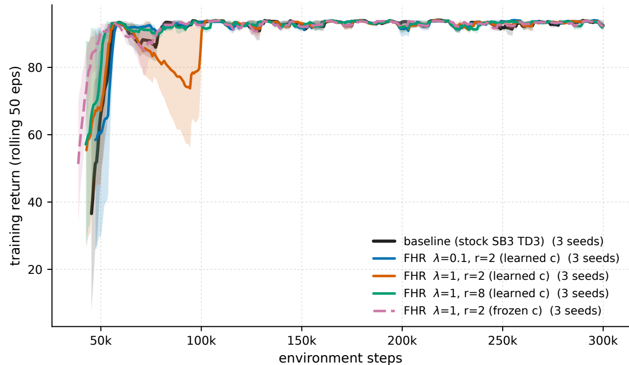
MountainCarContinuous-v0 - all arms (train)
