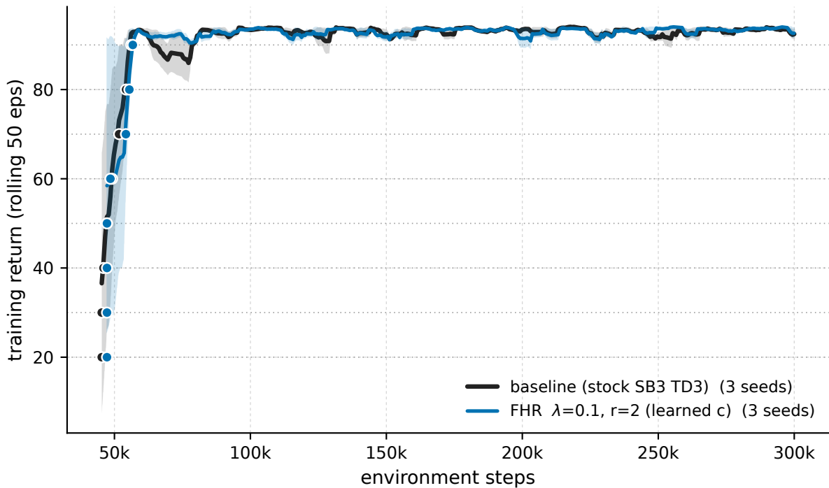
MountainCarContinuous-v0 - \lambda 0.1 \cdot r^2 vs baseline (training stream)
