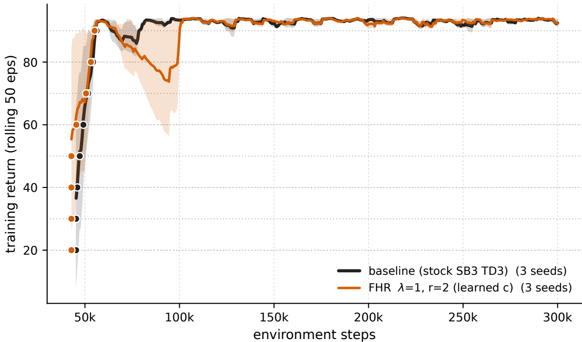
MountainCarContinuous-v0 - \lambda 1 \cdot r_2 vs baseline (training stream)
