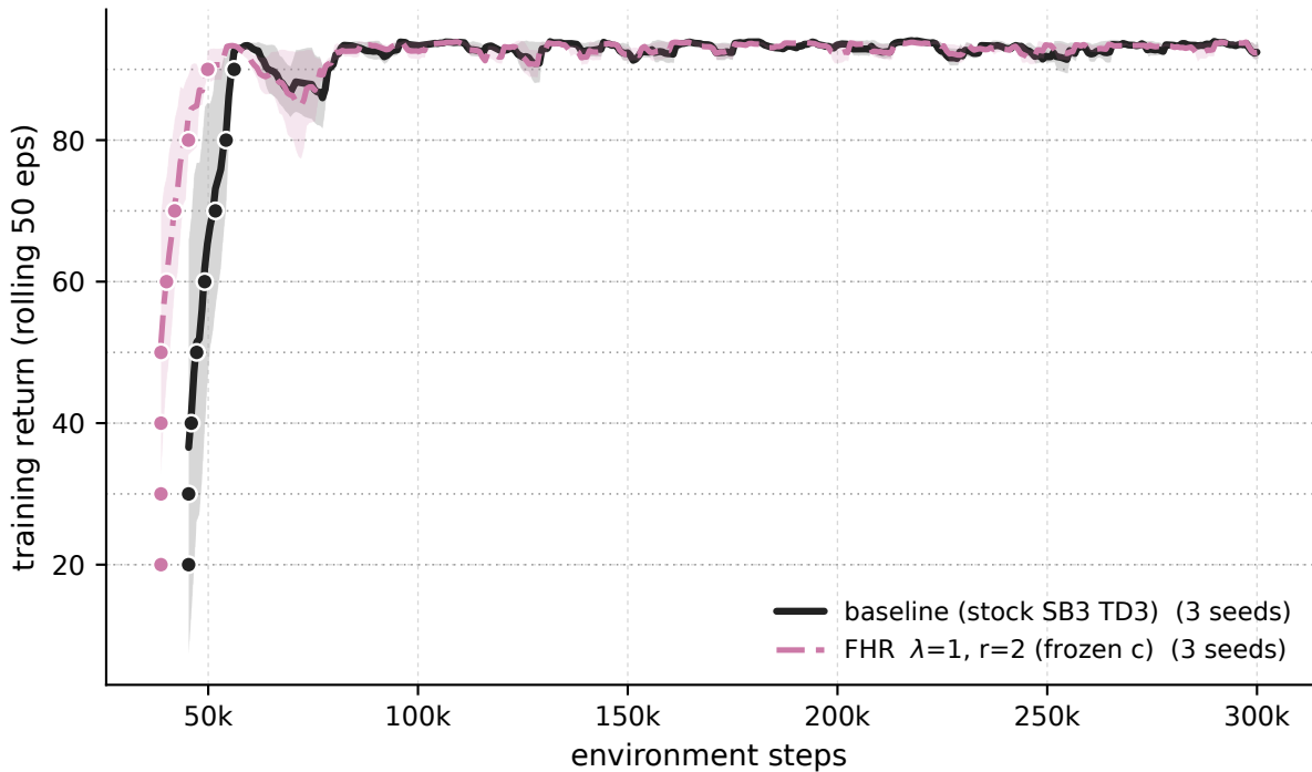
MountainCarContinuous-v0 - \lambda 1 \cdot r2 frozen-c vs baseline (training stream)
