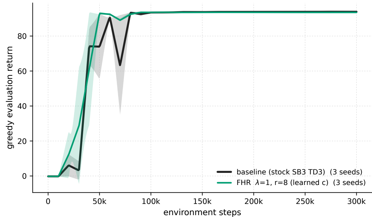
MountainCarContinuous-v0 - \lambda 1 \cdot r8 vs baseline (greedy eval)
