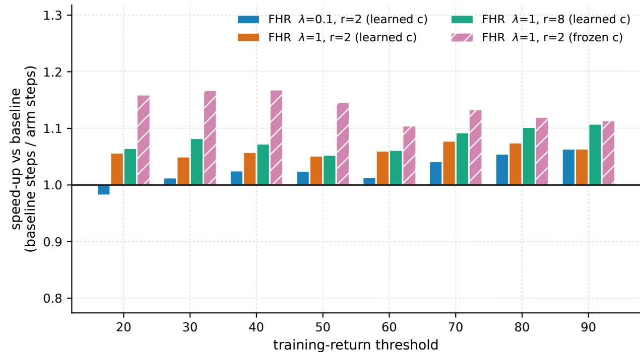
MountainCarContinuous-v0 - sample-efficiency ratio (thresholds all baseline seeds reached)
