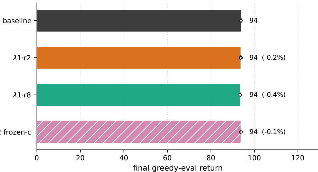
MountainCarContinuous-v0 - final return, \lambda = 1 vs baseline
