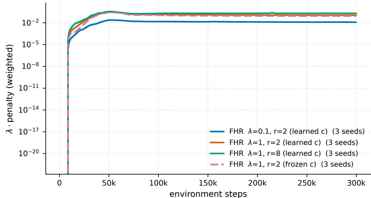
MountainCarContinuous-v0 - \lambda \cdot \text{penalty} (weighted)
