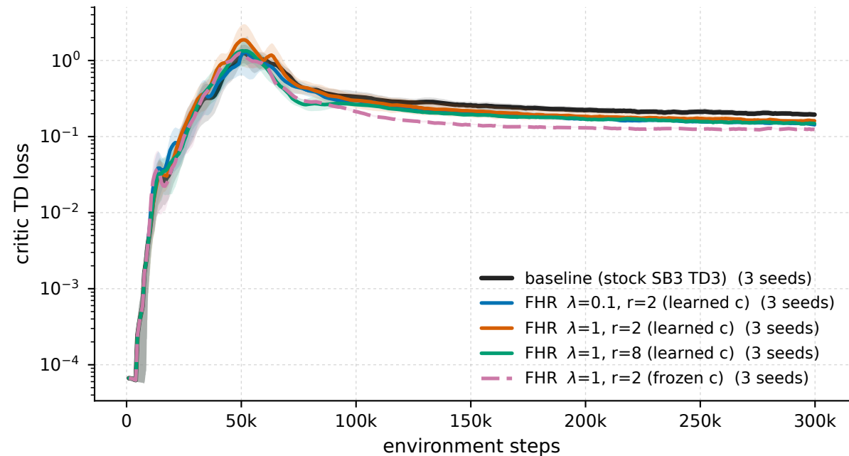
MountainCarContinuous-v0 - critic TD loss
