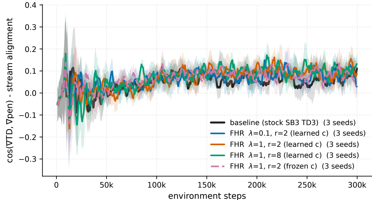
MountainCarContinuous-v0 - \cos(\nabla\text{T D}, \nabla\text{pen}) - stream alignment
