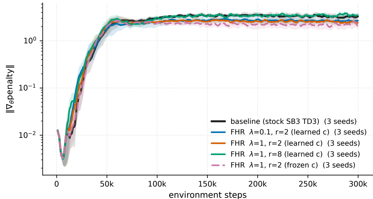
MountainCarContinuous-v0 - \|\nabla_{\theta}\text{penalty}\|
