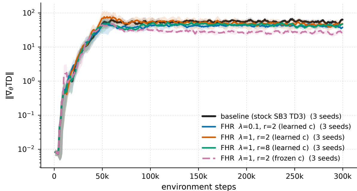
MountainCarContinuous-v0 - \|\nabla_{\theta}TD\|
