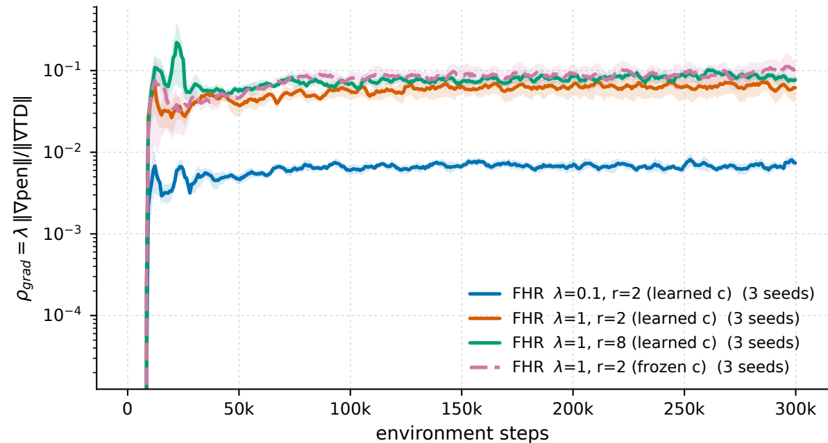
MountainCarContinuous-v0 - \rho_{grad} = \lambda \|\nabla pen\|/\|\nabla TD\|
