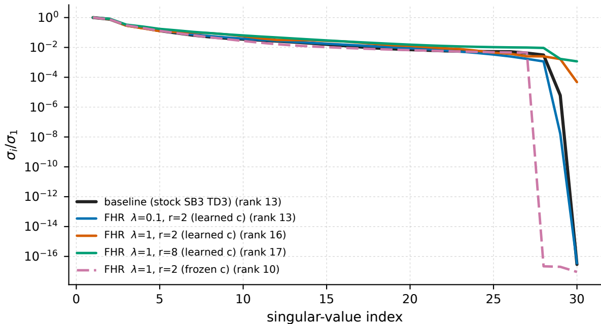
MountainCarContinuous-v0 - Hankel( \pi(s_t)_0 ) of the final policy (action dim 0)
