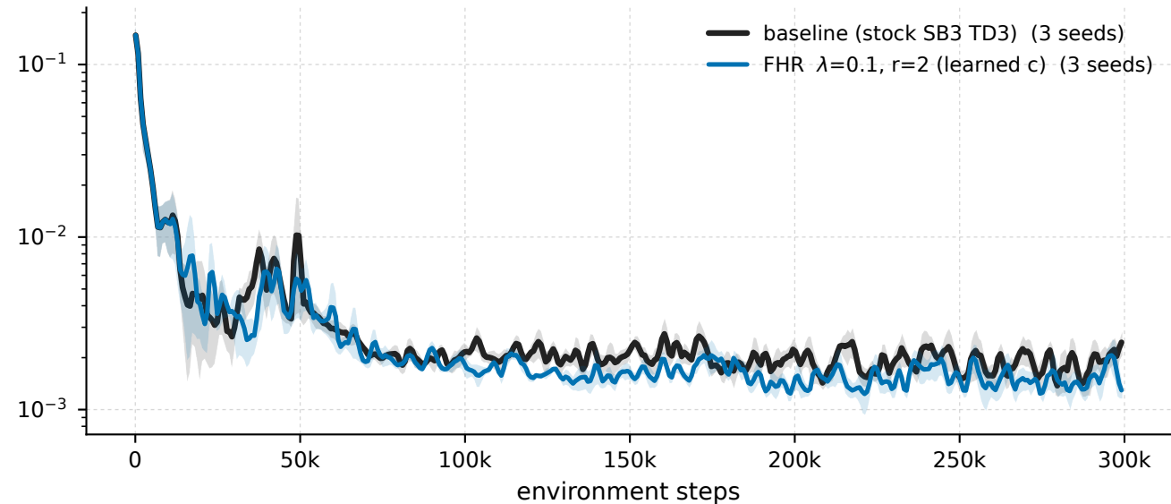
MountainCarContinuous-v0 - \lambda 0.1 \cdot r_2 vs baseline, penalised windows penalty-block tail \sigma_{r+1}/\sigma_1
