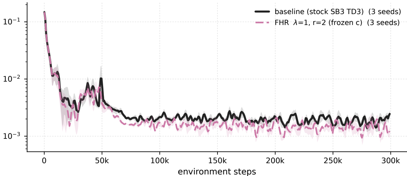
MountainCarContinuous-v0 - \lambda 1 \cdot r_2 frozen-c vs baseline, penalised windows penalty-block tail \sigma_{r+1}/\sigma_1
