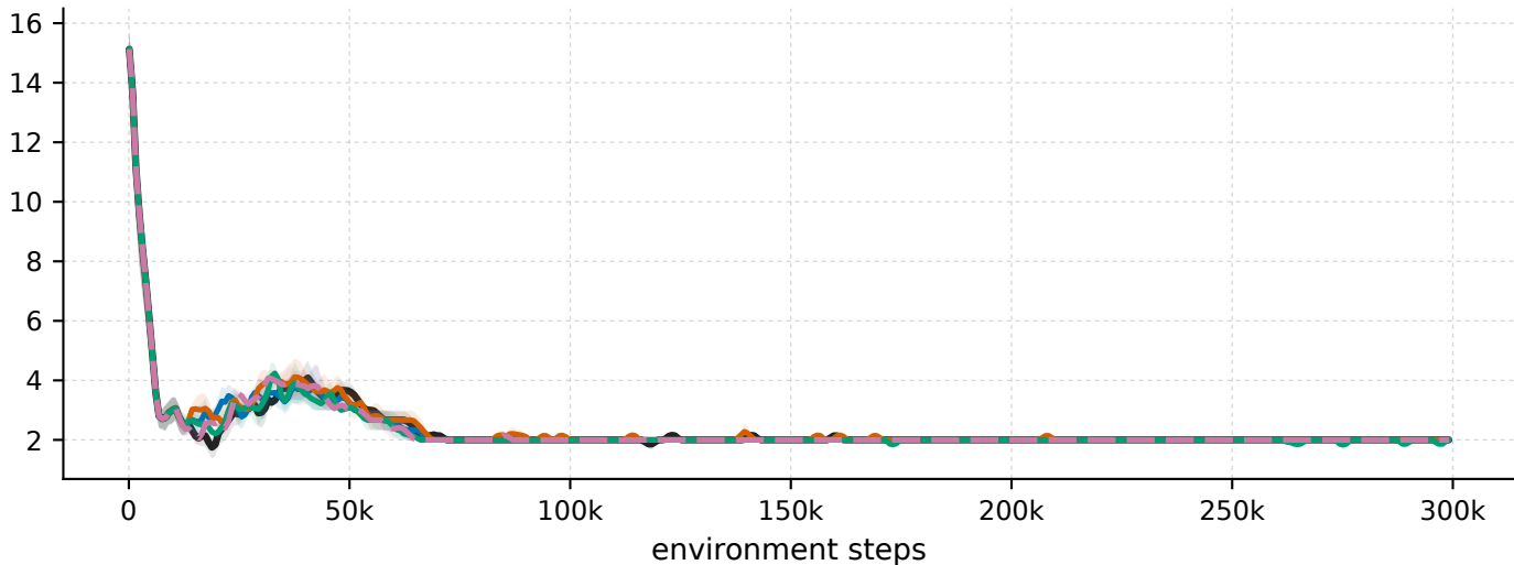
MountainCarContinuous-v0 - penalised windows, all arms energy rank @ 99.9%
