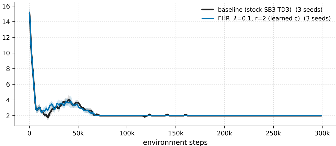
MountainCarContinuous-v0 - \lambda 0.1 \cdot r^2 vs baseline, penalised windows energy rank @ 99.9%
