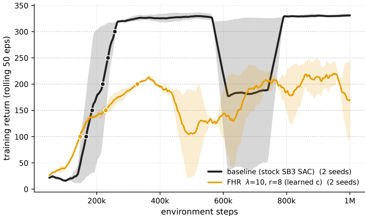
Swimmer-v5 - \lambda 10 \cdot r8 vs baseline (training stream)
