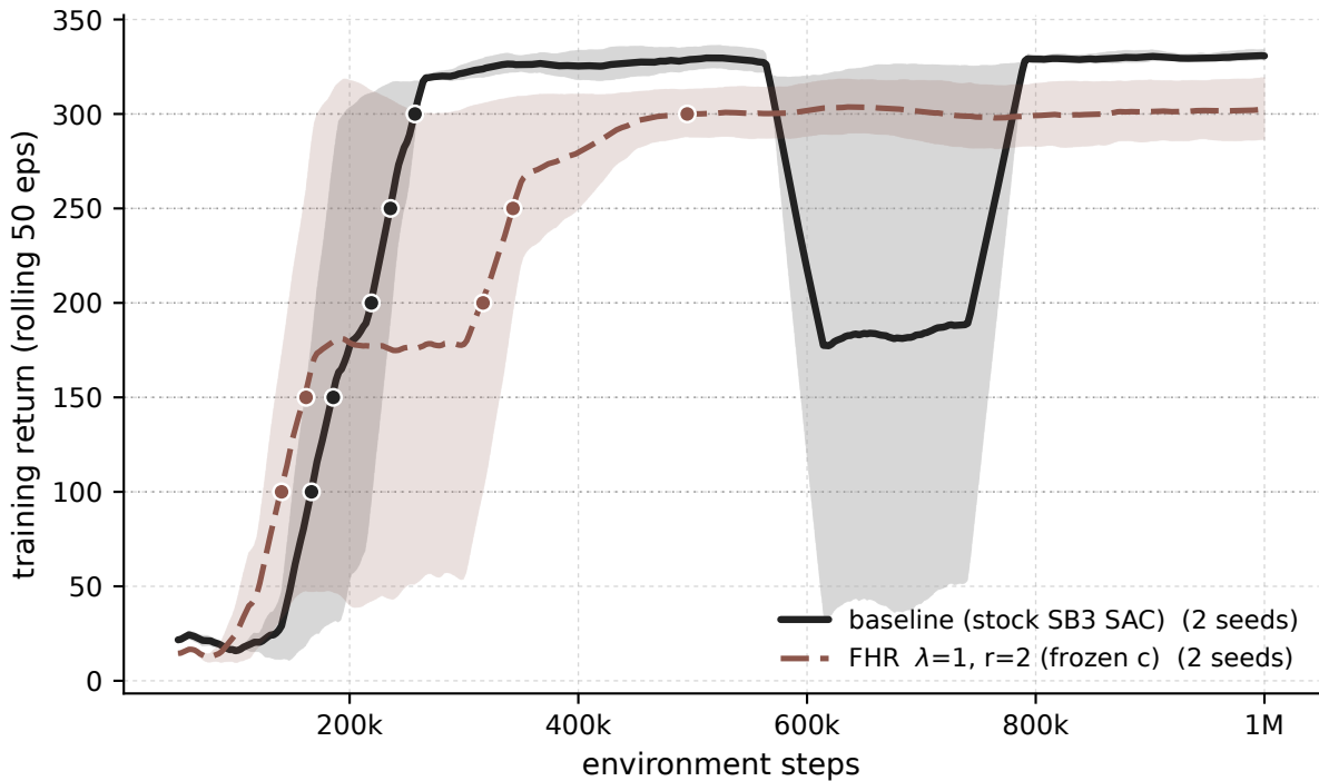
Swimmer-v5 - \lambda=1, r=2 frozen-c vs baseline (training stream)
