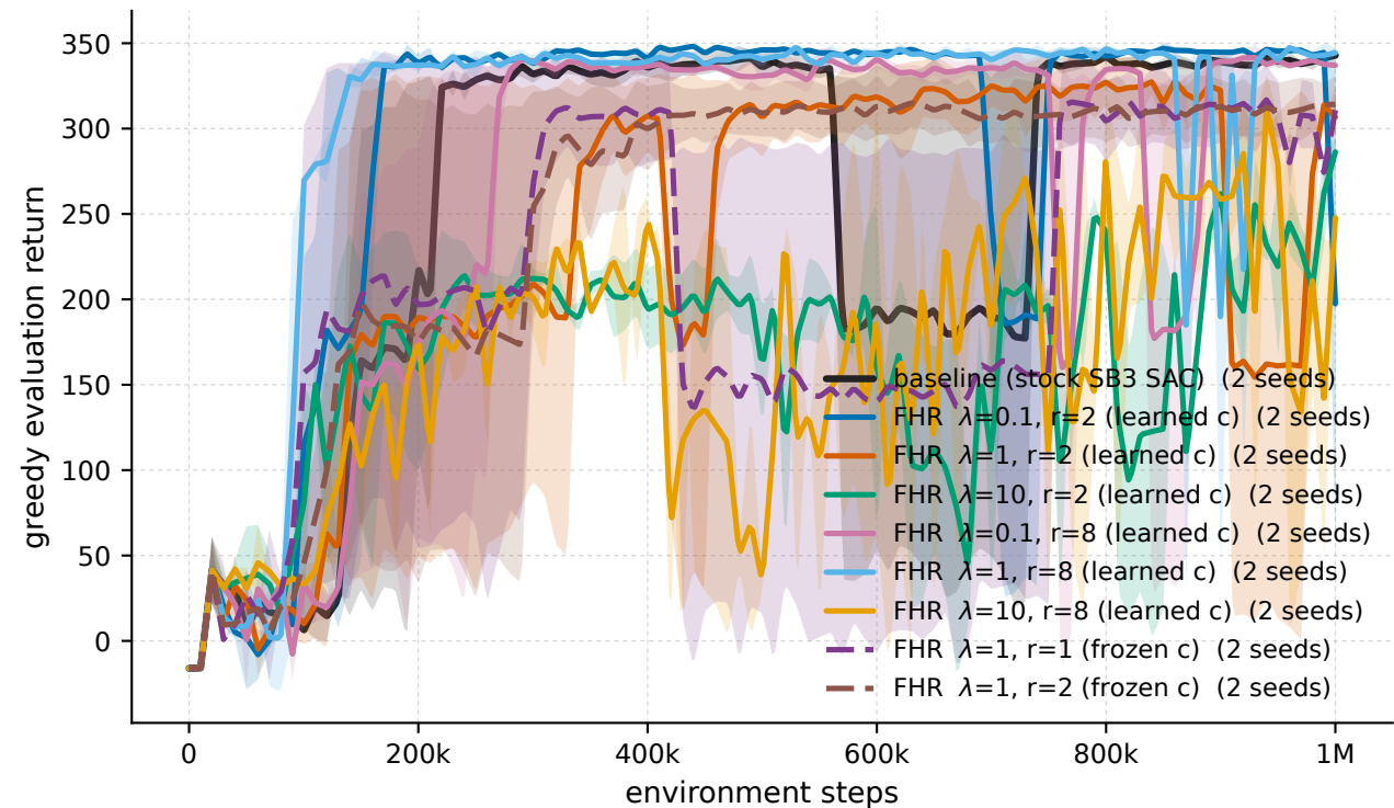
Swimmer-v5 - all arms (eval)
