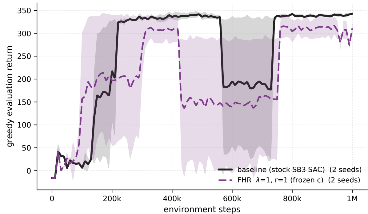
Swimmer-v5 - \lambda 1 \cdot r1 frozen-c vs baseline (greedy eval)
