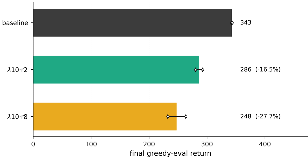
Swimmer-v5 - final return, \lambda = 10 vs baseline
