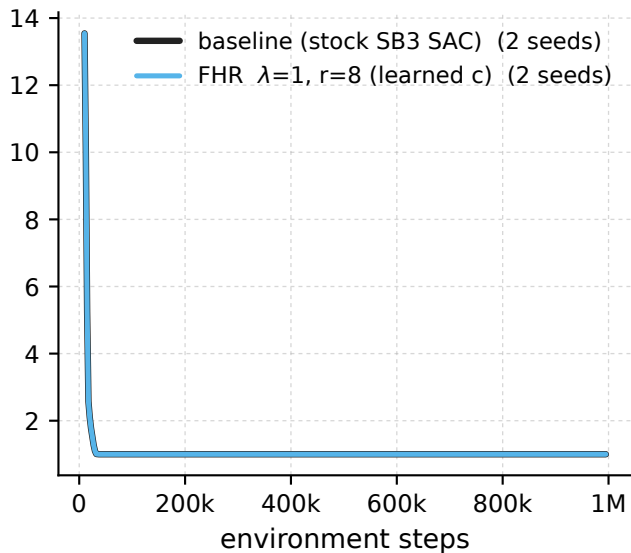
Swimmer-v5 - \lambda 1 \cdot r_8 vs baseline, penalised-window Hankel spectrum energy rank @ 99.9%
