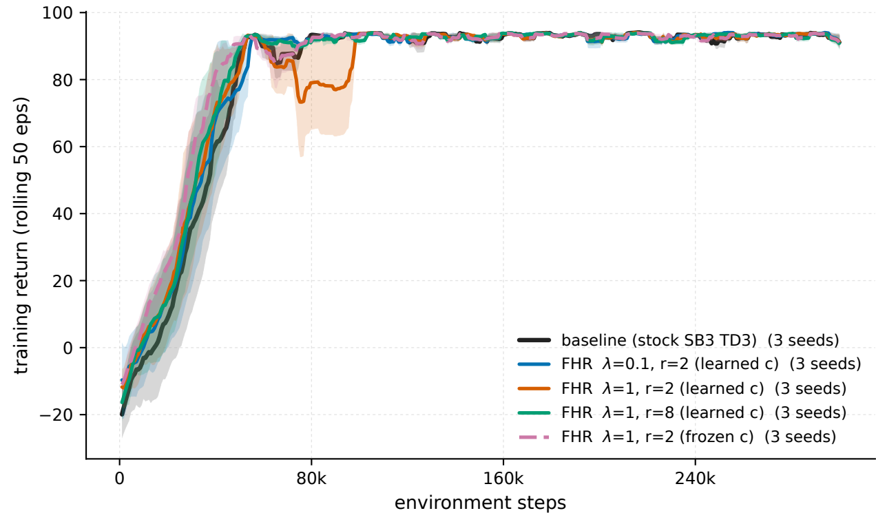
MountainCarContinuous-v0 - all arms (train)
