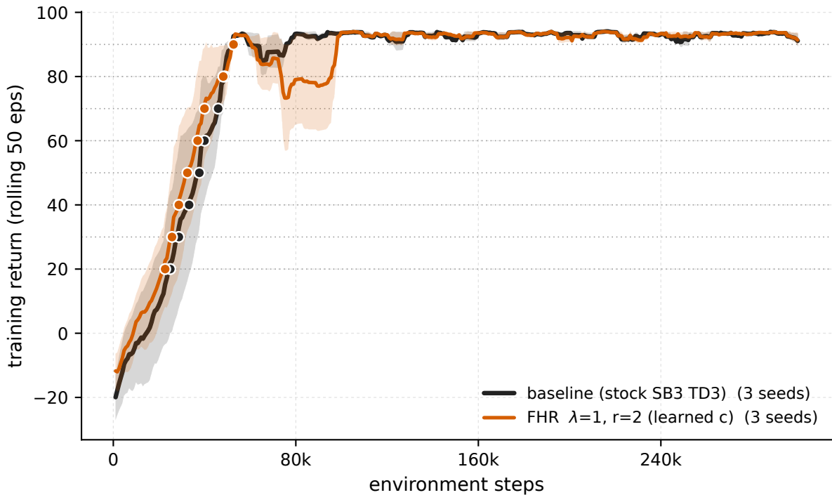
MountainCarContinuous-v0 - \lambda 1 \cdot r_2 vs baseline (training stream)
