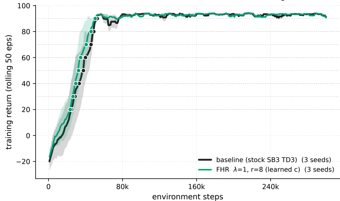
MountainCarContinuous-v0 - \lambda 1 \cdot r8 vs baseline (training stream)
