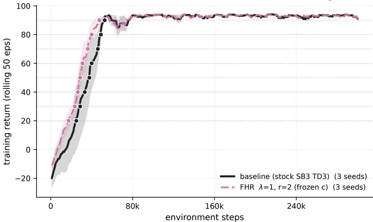
MountainCarContinuous-v0 - \lambda 1 \cdot r 2 frozen-c vs baseline (training stream)
