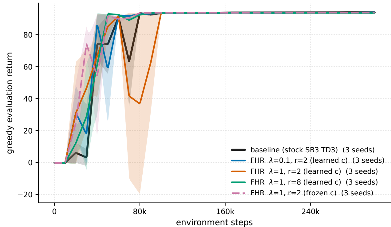
MountainCarContinuous-v0 - all arms (eval)
