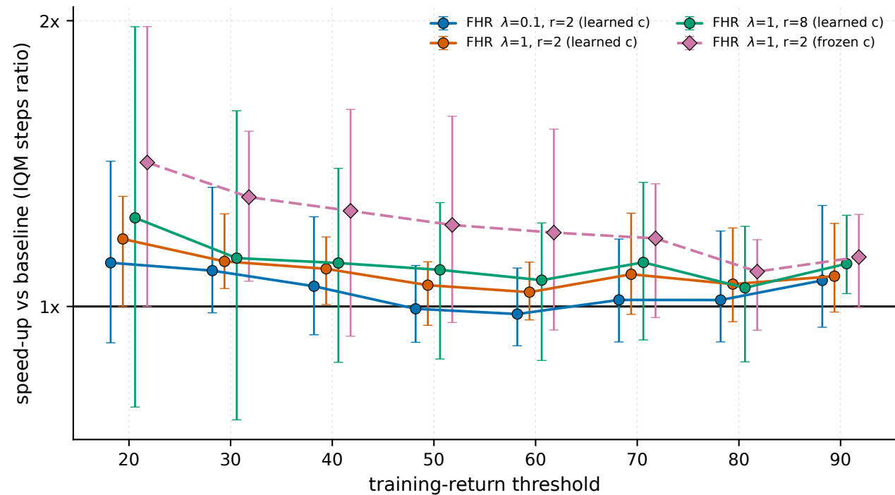
MountainCarContinuous-v0 - paired-bootstrap speed-up (95% CI); 'k/n' = seeds that reached the bar
