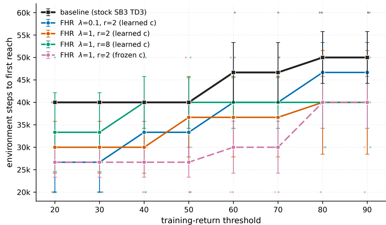
MountainCarContinuous-v0 - sample efficiency, greedy-eval stream (mean \pm 1 s.e.m.)
