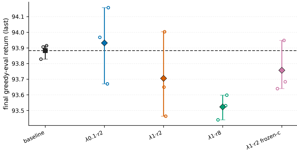
MountainCarContinuous-v0 - final return per arm: seeds (o), IQM with 95% bootstrap CI; dashed = baseline IQM
