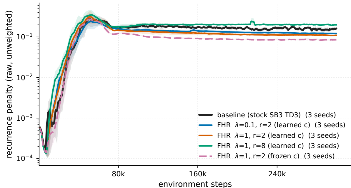
MountainCarContinuous-v0 - recurrence penalty (raw, unweighted)
