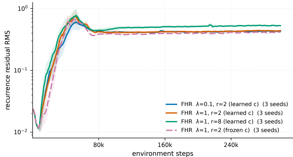
MountainCarContinuous-v0 - recurrence residual RMS
