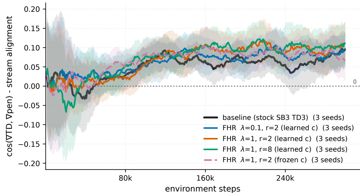
MountainCarContinuous-v0 - \cos(\nabla\text{T D}, \nabla\text{pen}) - stream alignment
