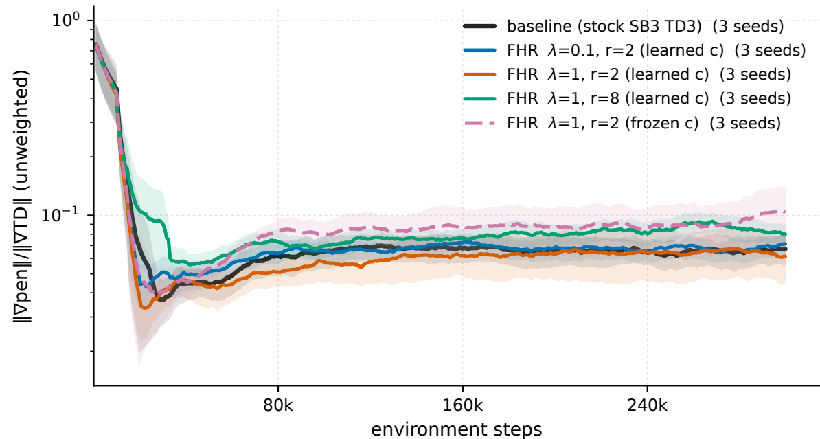
MountainCarContinuous-v0 - \|\nabla_{\text{pen}}\|/\|\nabla_{\text{TD}}\| (unweighted)
