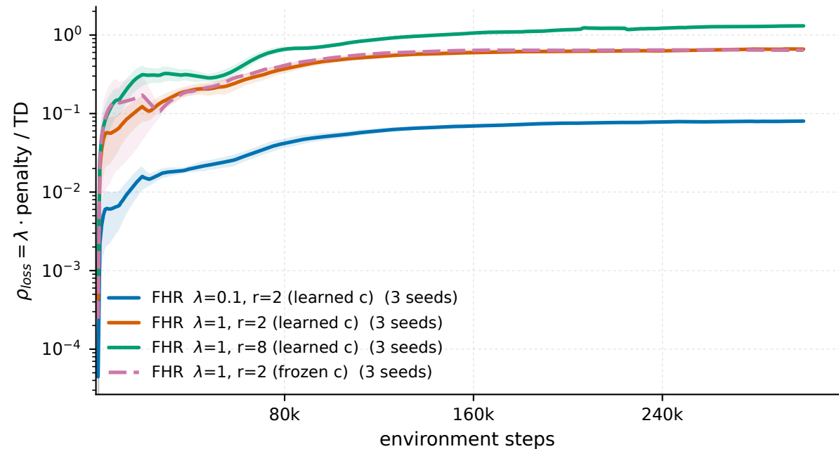
MountainCarContinuous-v0 - \rho_{loss} = \lambda \cdot \text{penalty} / \text{TD}
