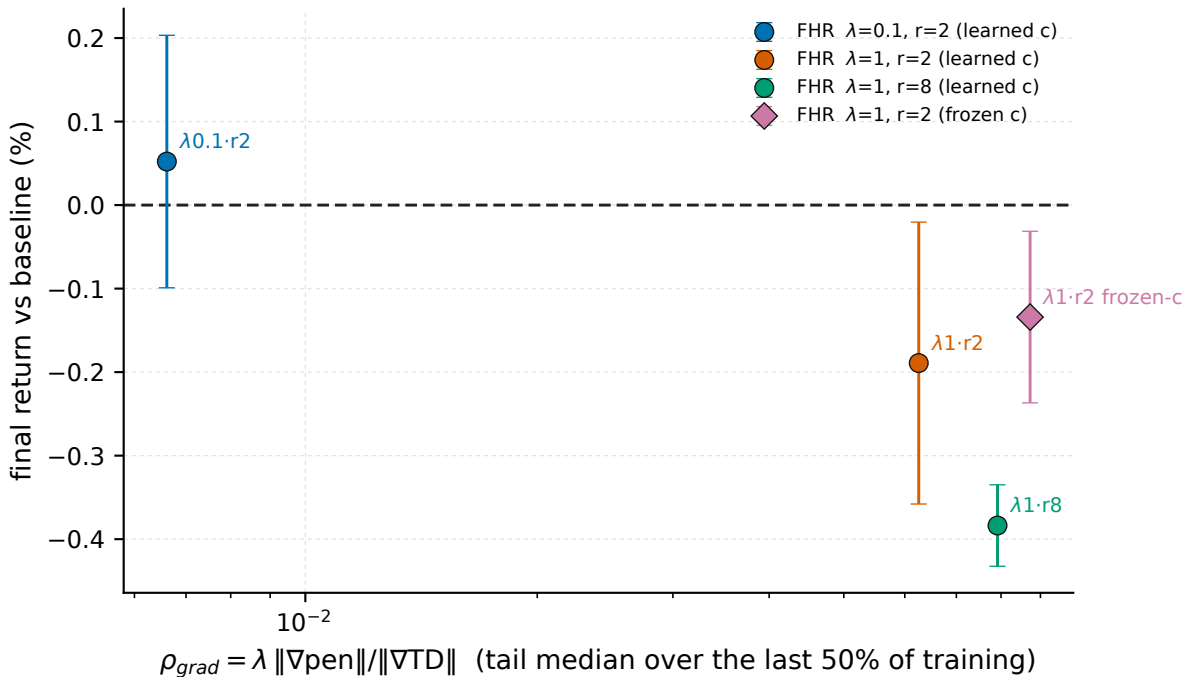
MountainCarContinuous-v0 - how hard the penalty pushes vs what it buys
