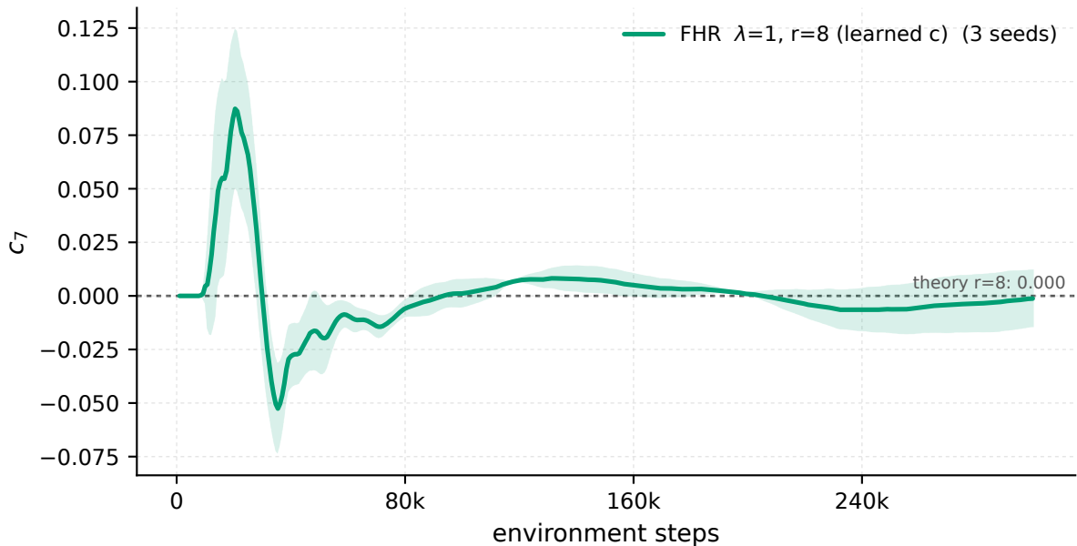
MountainCarContinuous-v0 - recurrence coefficient c_7 vs the Bellman theory value
